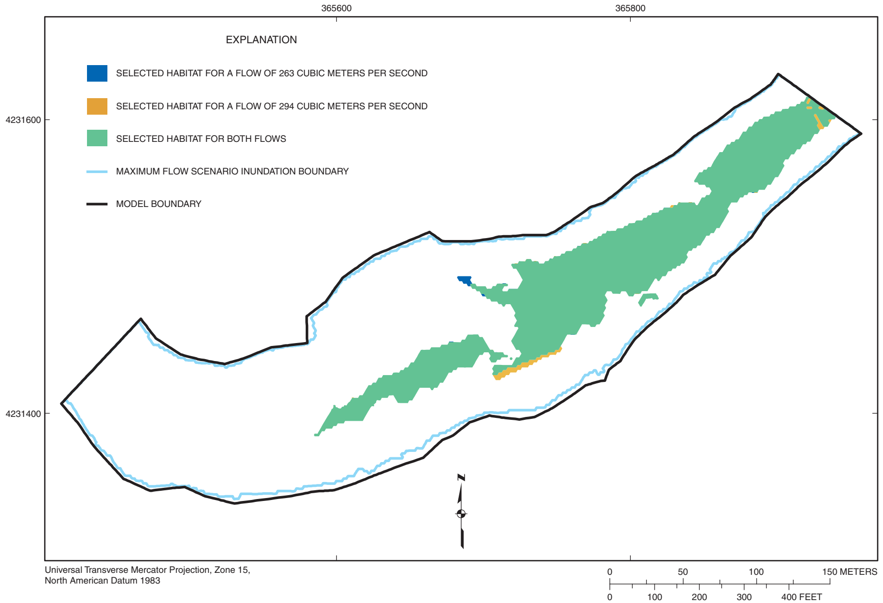
Figure 4-34. Selected habitat area distribution for habitat category 7 (paddlefish) at flows of 263 and 294 cubic meters per second at Marais des Cygnes River site MDC2.
